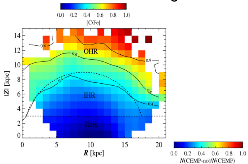
Carbonicity Map & Division of Inner and Outer Halo Regions
